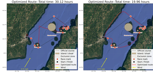
FIGURE 2. Optimized routes for the velocity-based relation (left) and acceleration-based (right) models.
